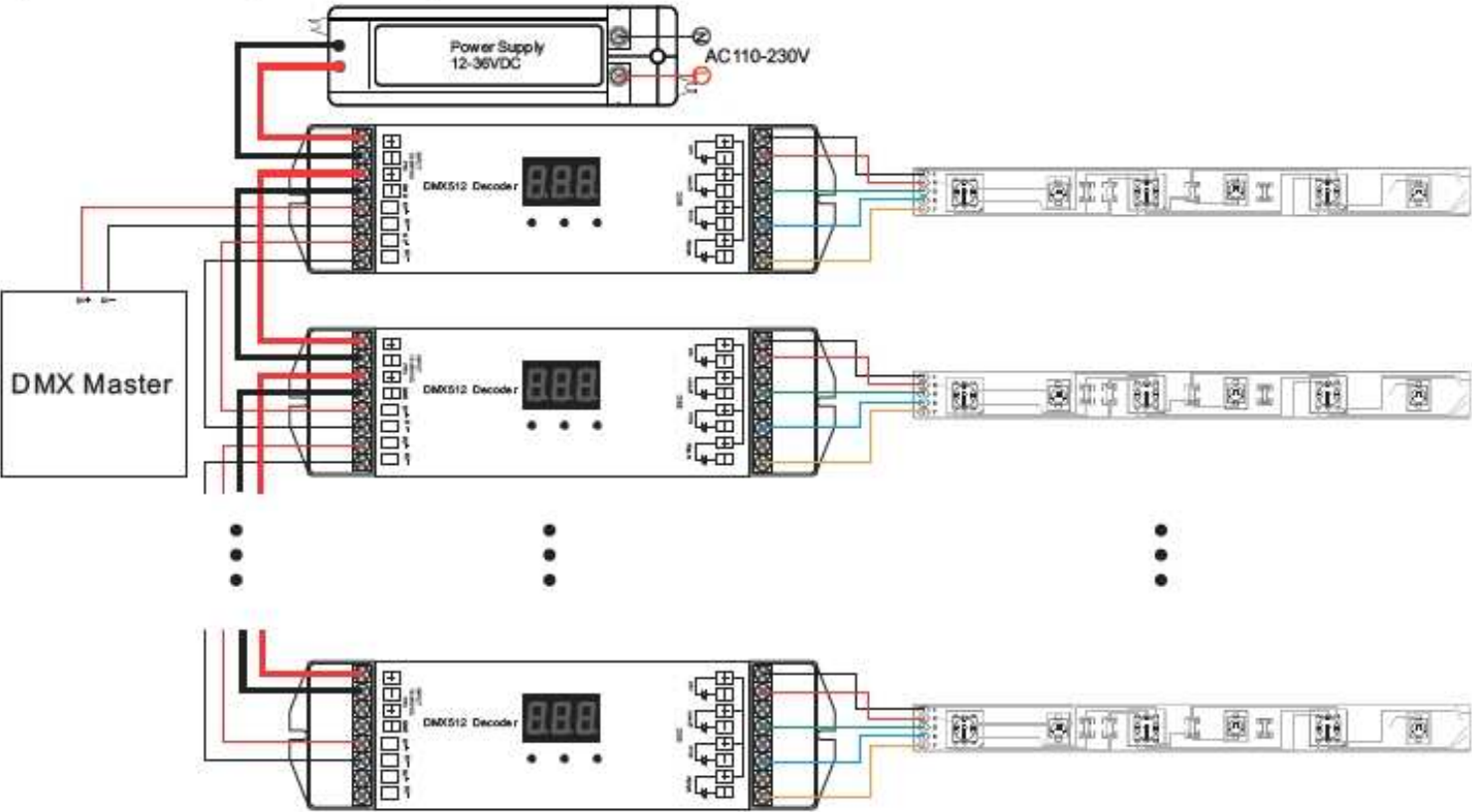
2)Connection Diagram for Multiple Units
